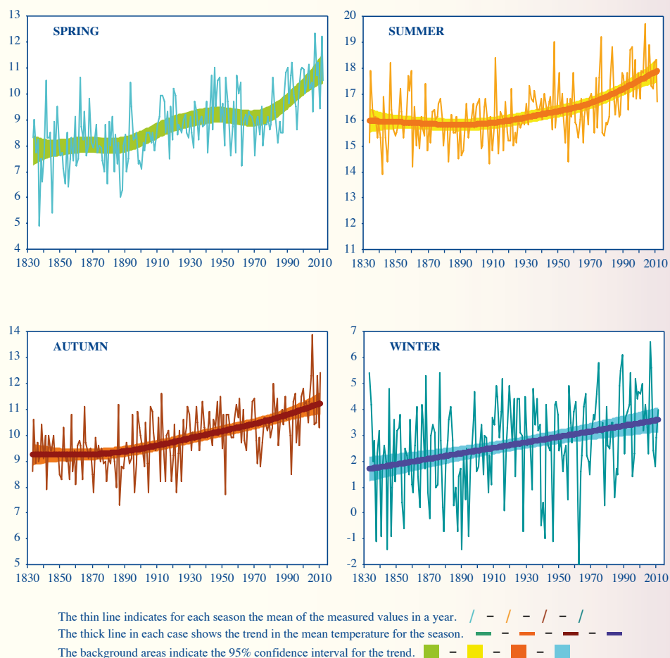
Figure 6.2 Mean temperature per season (°C) in Uccle, 1833-2012
