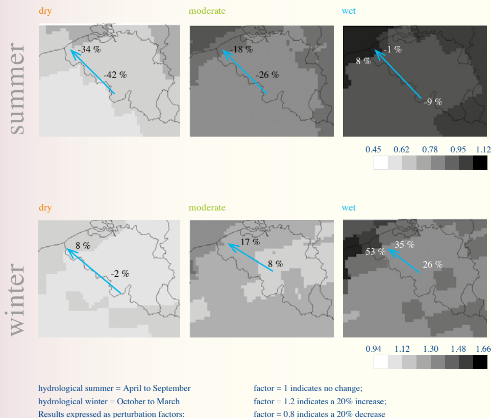
Figure 6.7 Regional differences for the seasonal average precipitation according to the three climate scenarios (Belgium, scenario period 2071-2100 compared to reference period 1961-1990)
